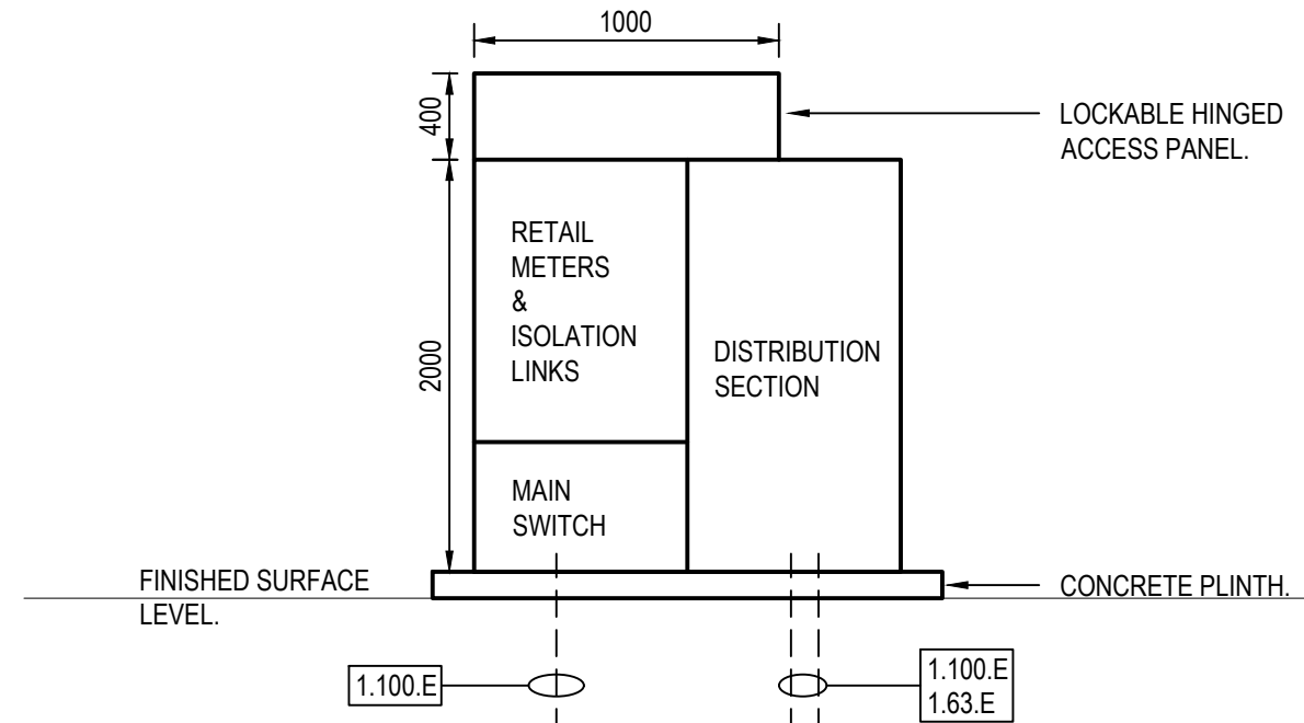
2 CONCEPT NEW MAIN SWITCHBOARD NOT TO SCALE
