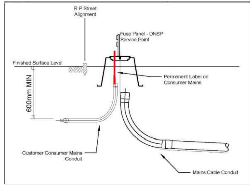
1 POINT OF SUPPLY CONNECTION NOT TO SCALE
