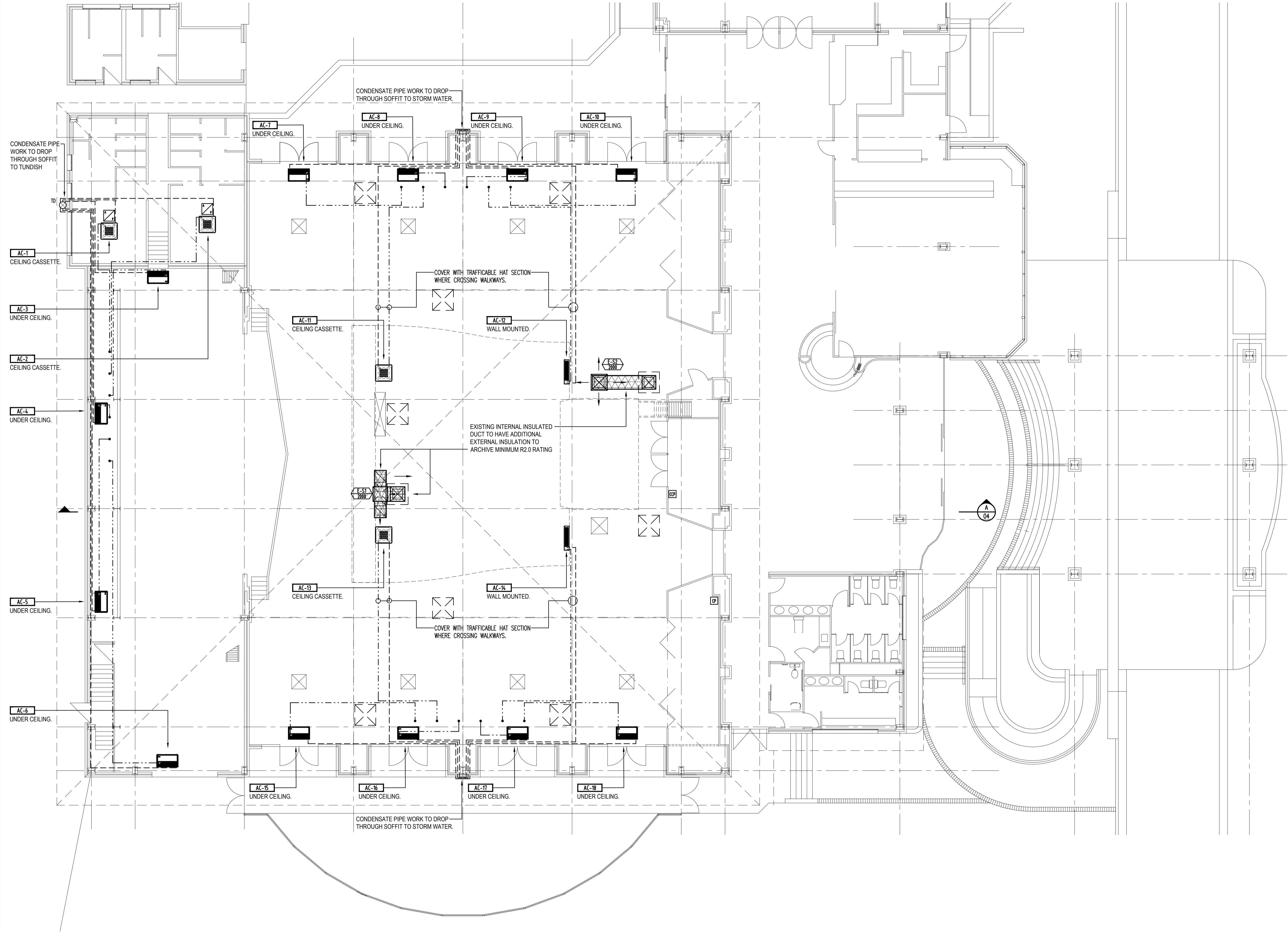
NEW AIR CONDITIONING AND VENTILATION LAYOUT SCALE - 1:100
